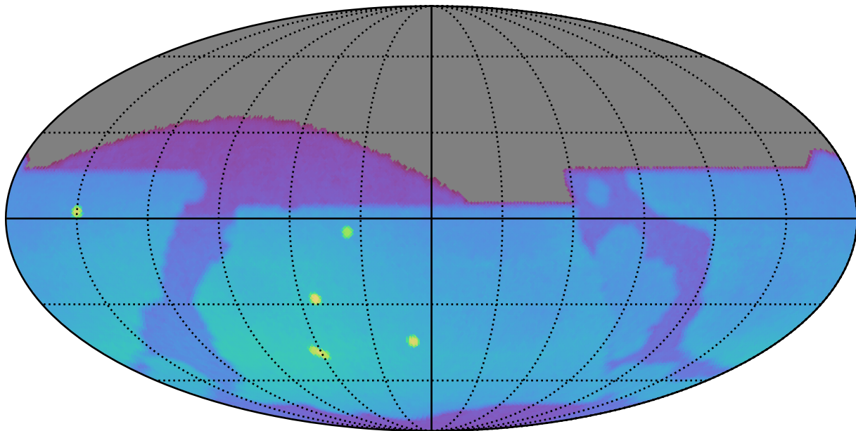
ddf_acor_sf15_lsf40_lsr50_v3.4_10yrs : Brown Dwarf, L4
