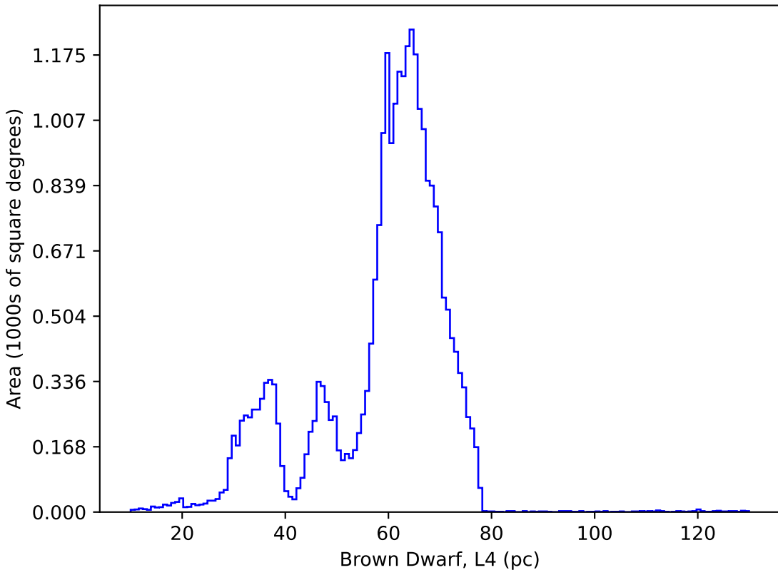
ddf_acor_sf15_lsf40_lsr50_v3.4_10yrs : Brown Dwarf, L4
