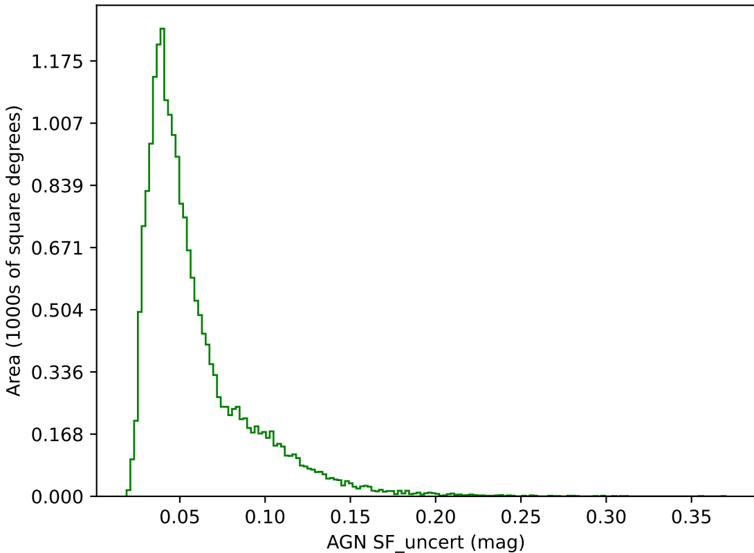
ddf_acor_sf15_lsf40_lsr50_v3.4_10yrs g band: AGN SF_uncert
