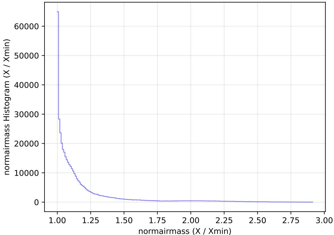
ddf_acor_sf15_lsf40_lsr50_v3.4_10yrs All sky z band: normairmass Histogram
