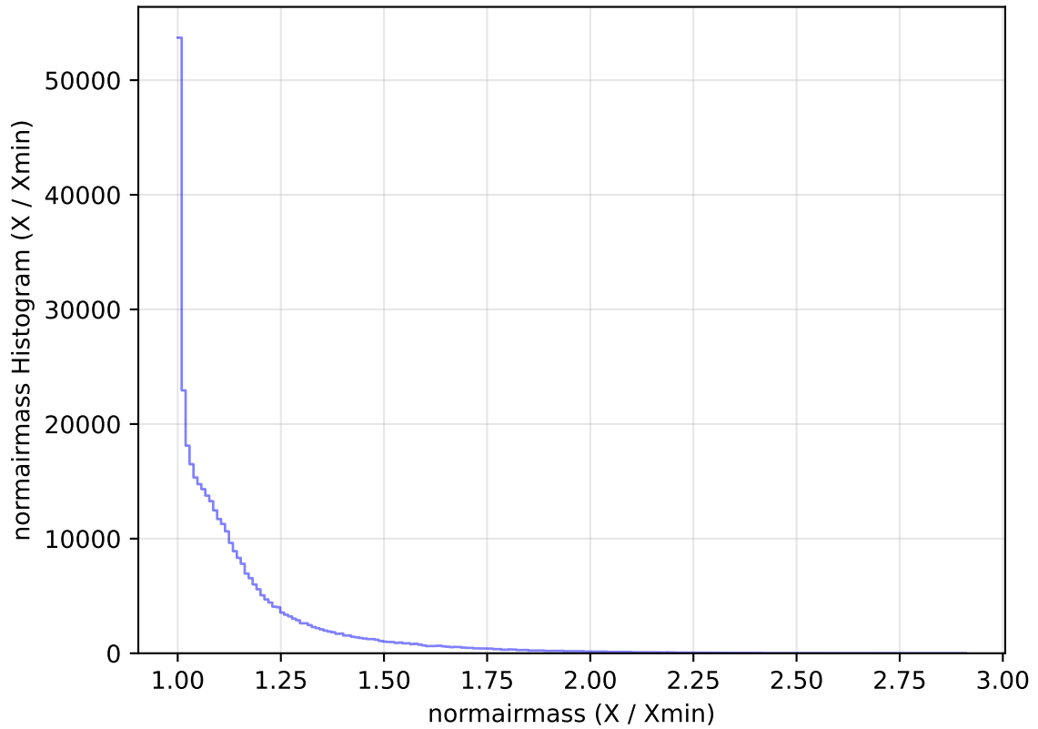
ddf_acor_sf15_lsf40_lsr50_v3.4_10yrs All sky y band: normairmass Histogram
