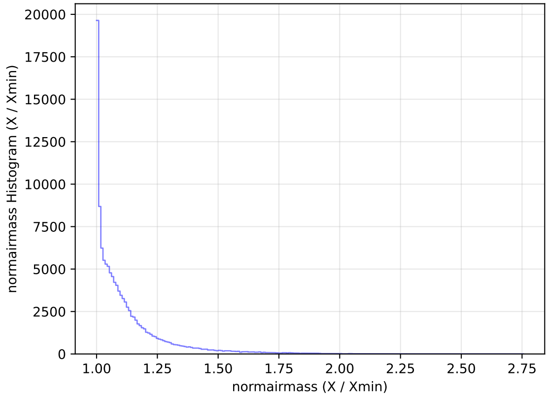
ddf_acor_sf15_lsf40_lsr50_v3.4_10yrs All sky u band: normairmass Histogram
