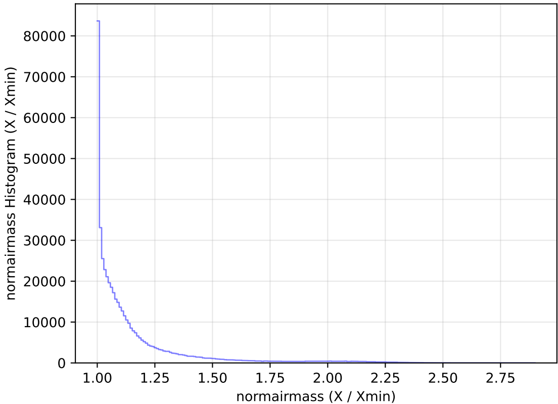
ddf_acor_sf15_lsf40_lsr50_v3.4_10yrs All sky r band: normairmass Histogram
