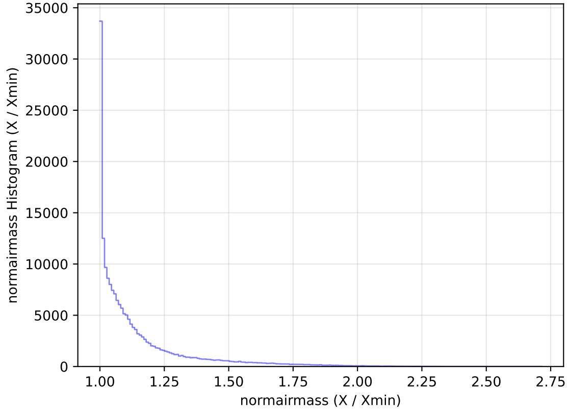
ddf_acor_sf15_lsf40_lsr50_v3.4_10yrs All sky g band: normairmass Histogram
