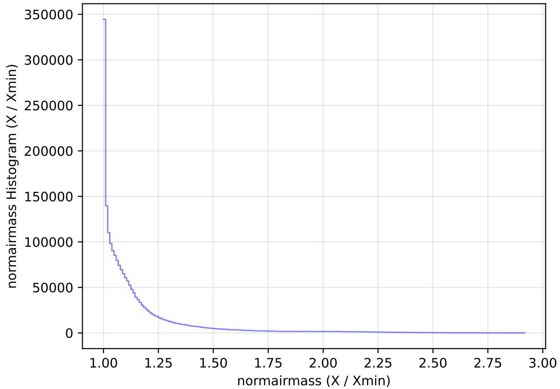
ddf_acor_sf15_lsf40_lsr50_v3.4_10yrs All sky all bands: normairmass Histogram
