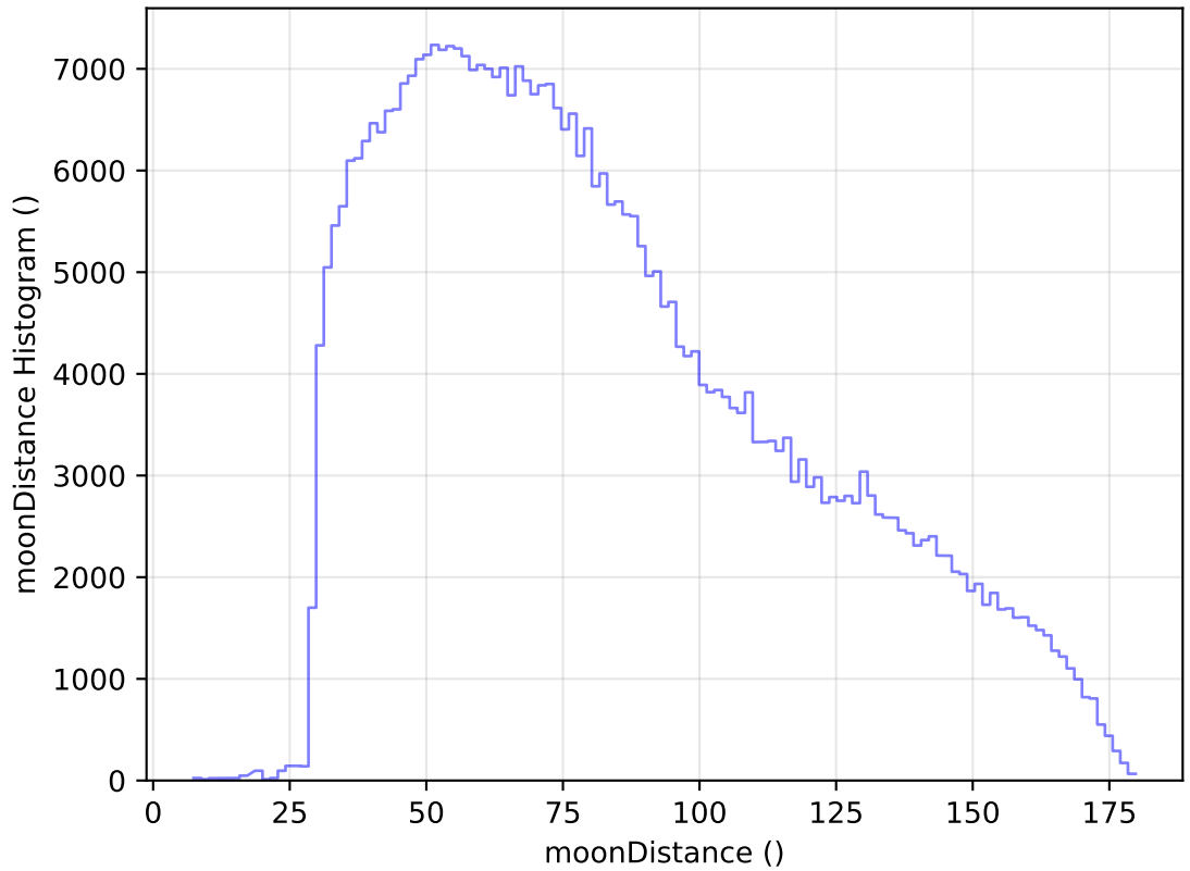
ddf_acor_sf15_lsf40_lsr50_v3.4_10yrs WFD z band: moonDistance Histogram
