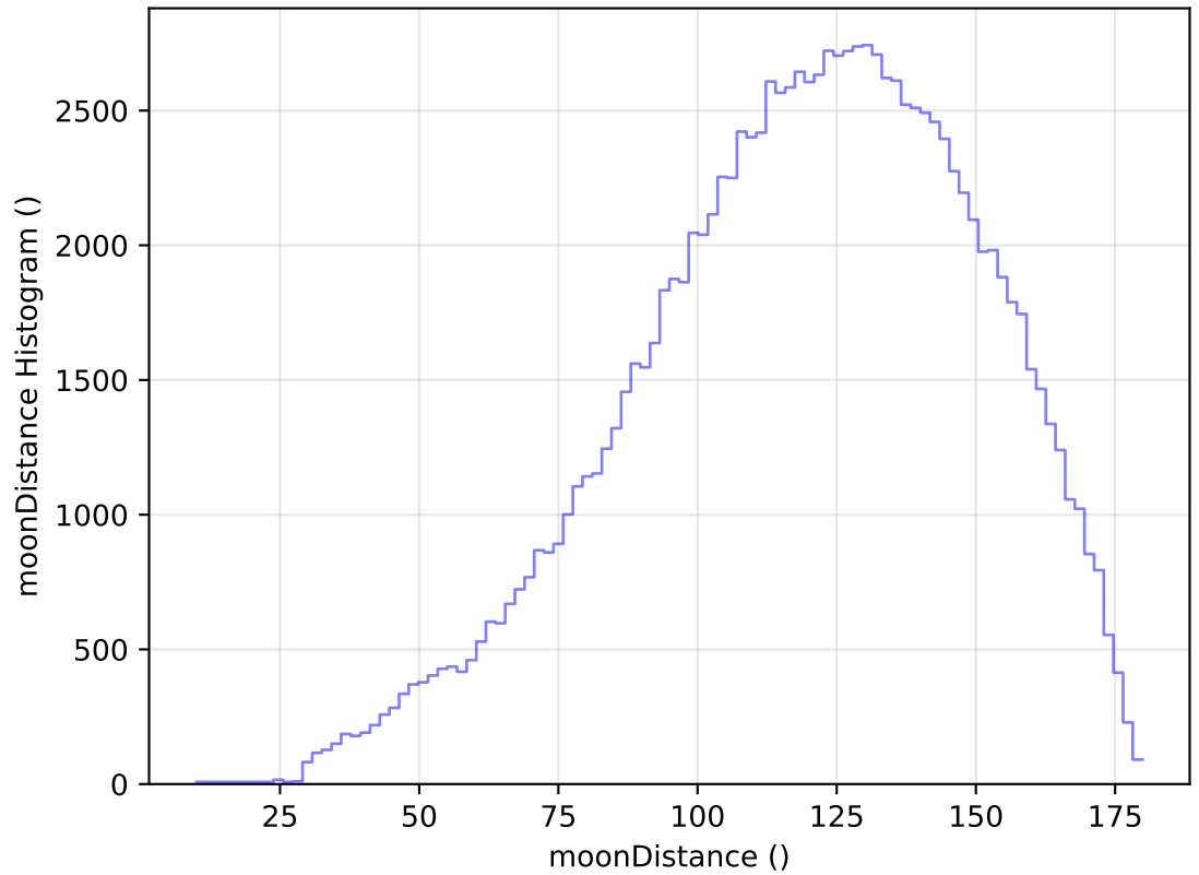
ddf_acor_sf15_lsf40_lsr50_v3.4_10yrs WFD u band: moonDistance Histogram
