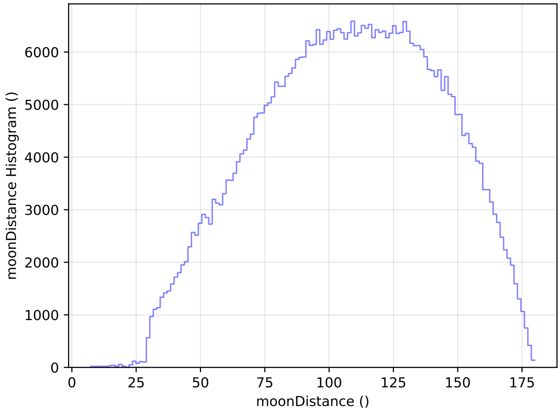
ddf_acor_sf15_lsf40_lsr50_v3.4_10yrs WFD r band: moonDistance Histogram
