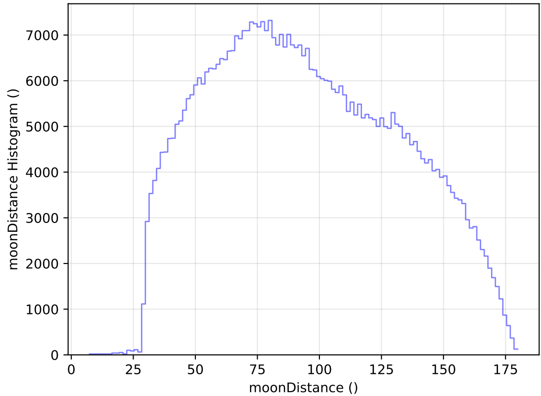
ddf_acor_sf15_lsf40_lsr50_v3.4_10yrs WFD i band: moonDistance Histogram
