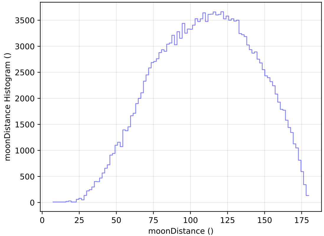
ddf_acor_sf15_lsf40_lsr50_v3.4_10yrs WFD g band: moonDistance Histogram
