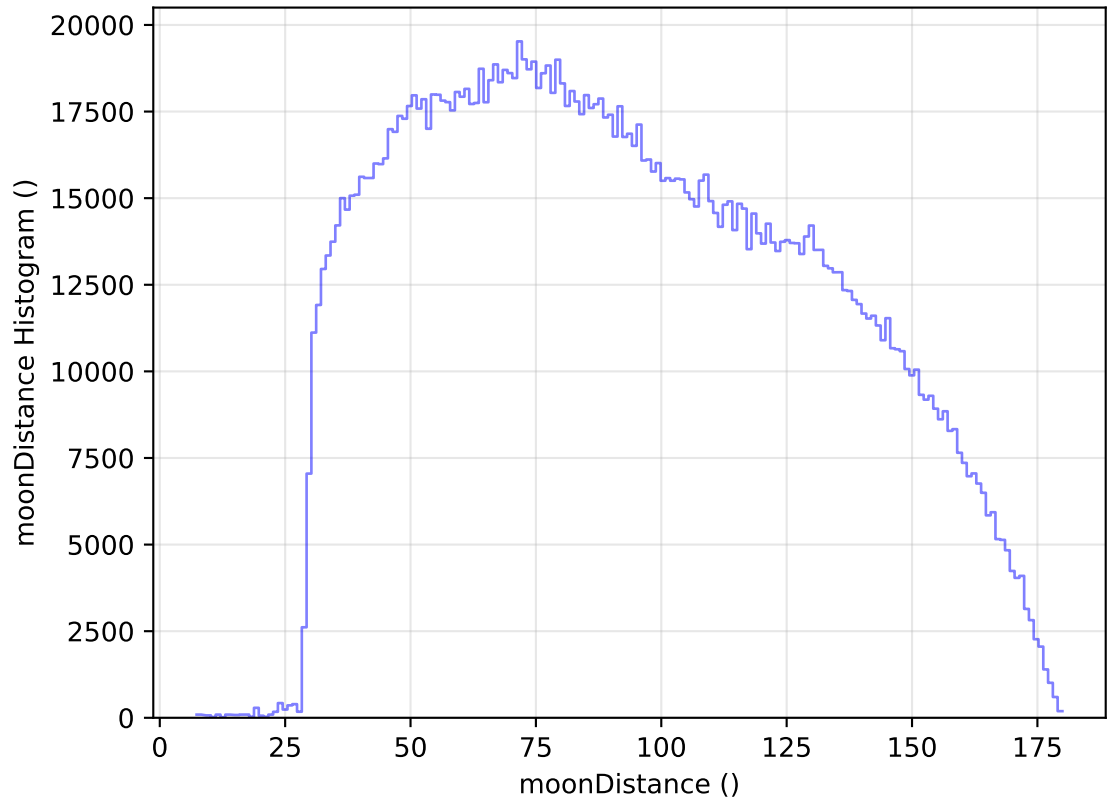
ddf_acor_sf15_lsf40_lsr50_v3.4_10yrs WFD all bands: moonDistance Histogram
