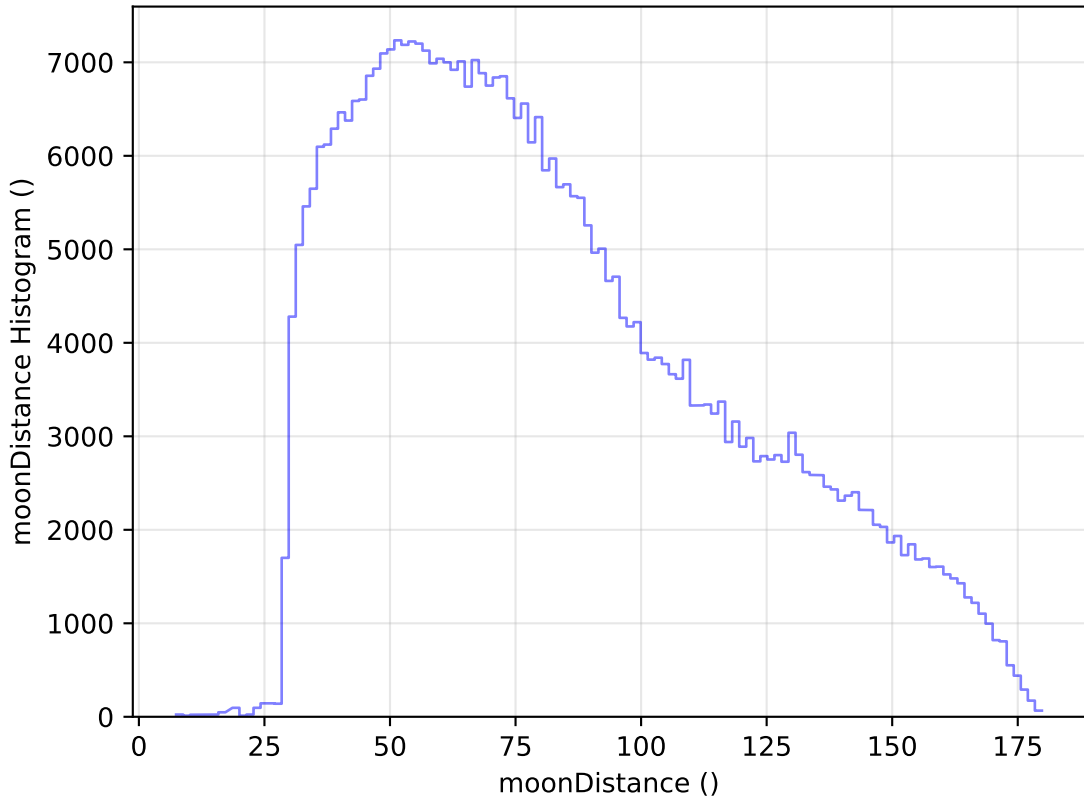
ddf_acor_sf15_lsf40_lsr50_v3.4_10yrs All sky z band: moonDistance Histogram
