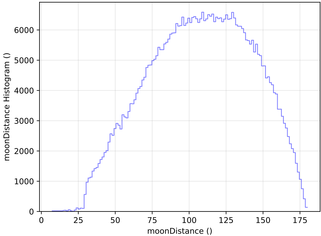
ddf_acor_sf15_lsf40_lsr50_v3.4_10yrs All sky r band: moonDistance Histogram
