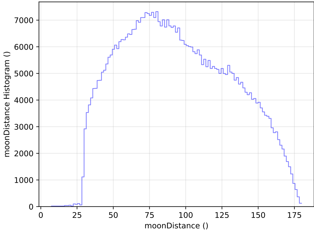
ddf_acor_sf15_lsf40_lsr50_v3.4_10yrs All sky i band: moonDistance Histogram
