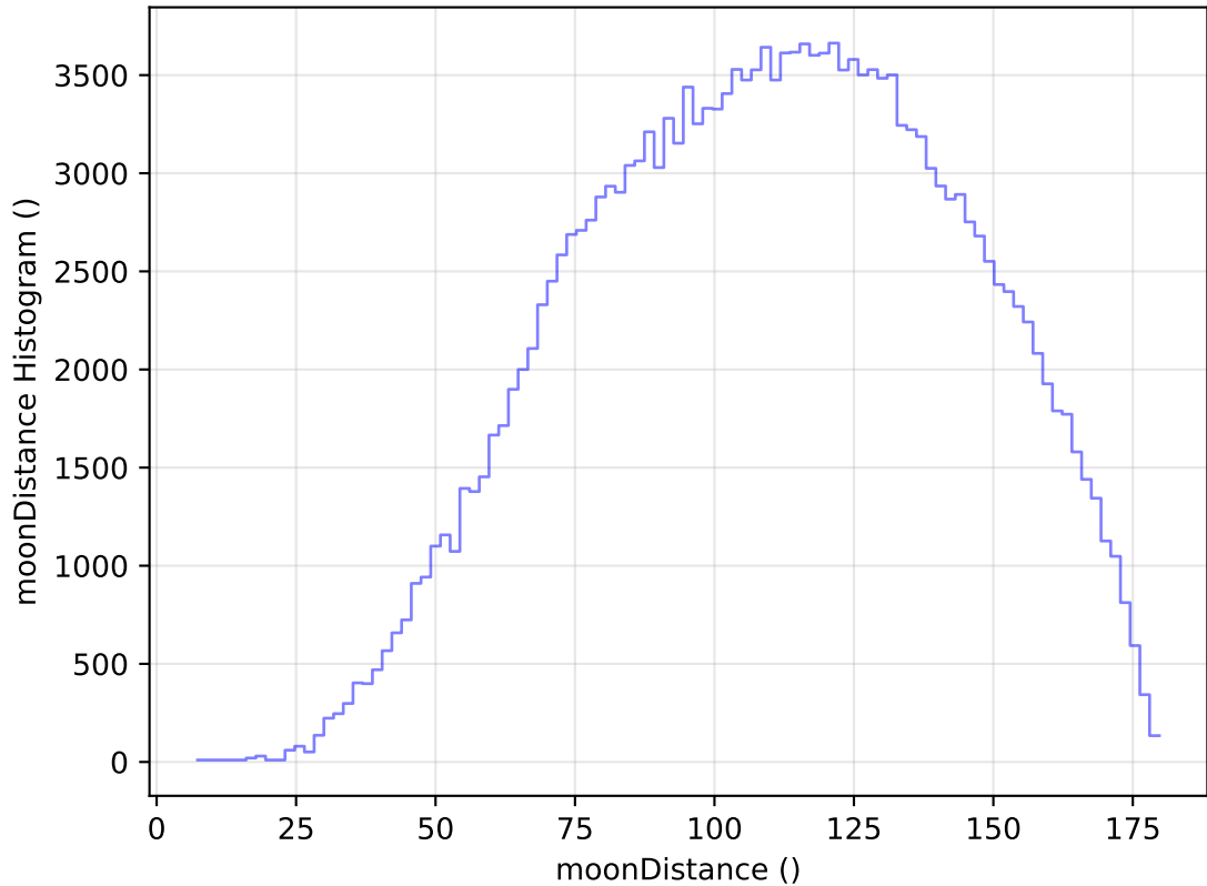
ddf_acor_sf15_lsf40_lsr50_v3.4_10yrs All sky g band: moonDistance Histogram
