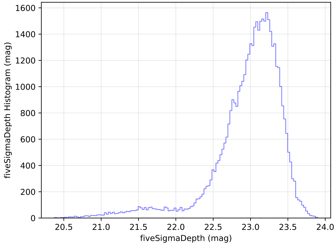
ddf_acor_sf15_lsf40_lsr50_v3.4_10yrs Yr 1 z band: fiveSigmaDepth Histogram
