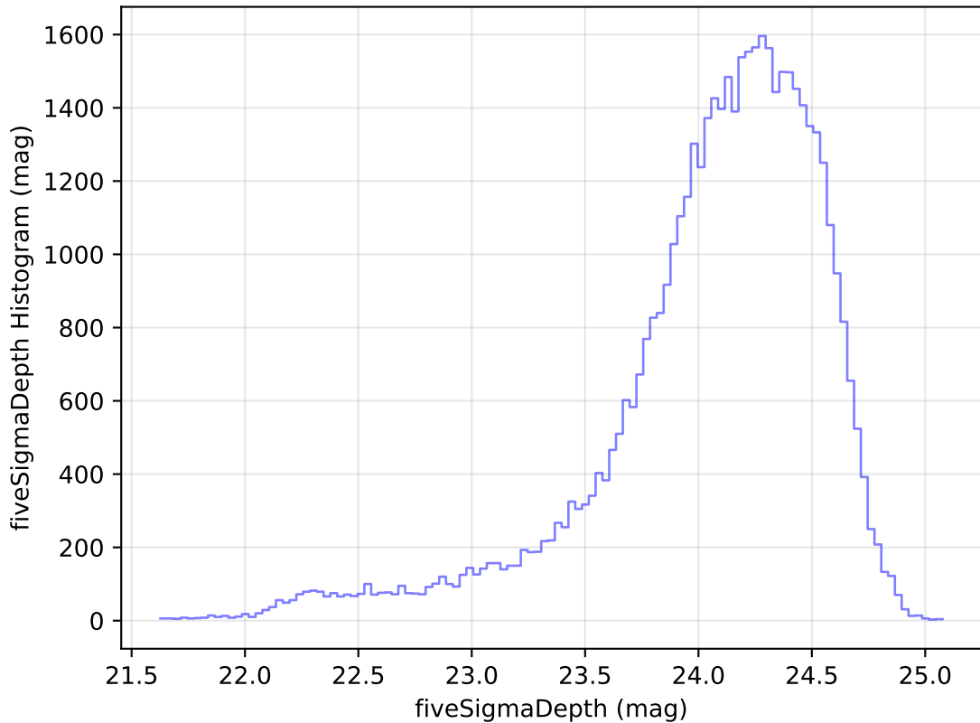
ddf_acor_sf15_lsf40_lsr50_v3.4_10yrs Yr 1 r band: fiveSigmaDepth Histogram
