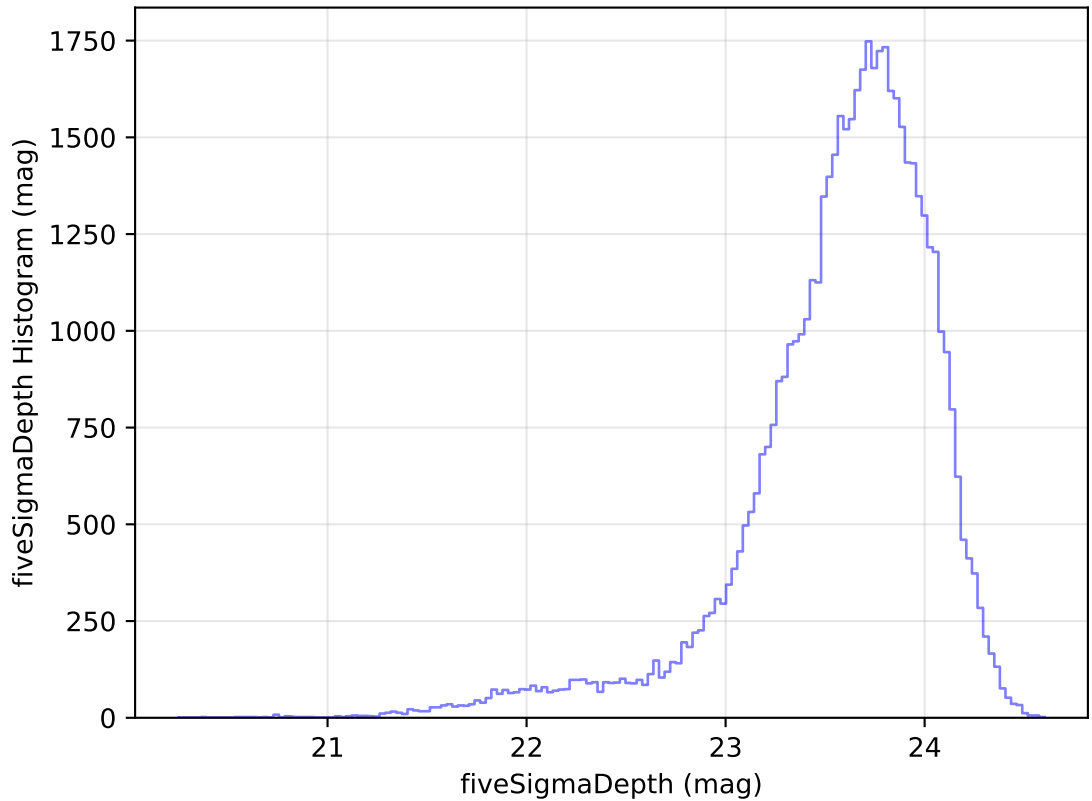
ddf_acor_sf15_lsf40_lsr50_v3.4_10yrs Yr 1 i band: fiveSigmaDepth Histogram
