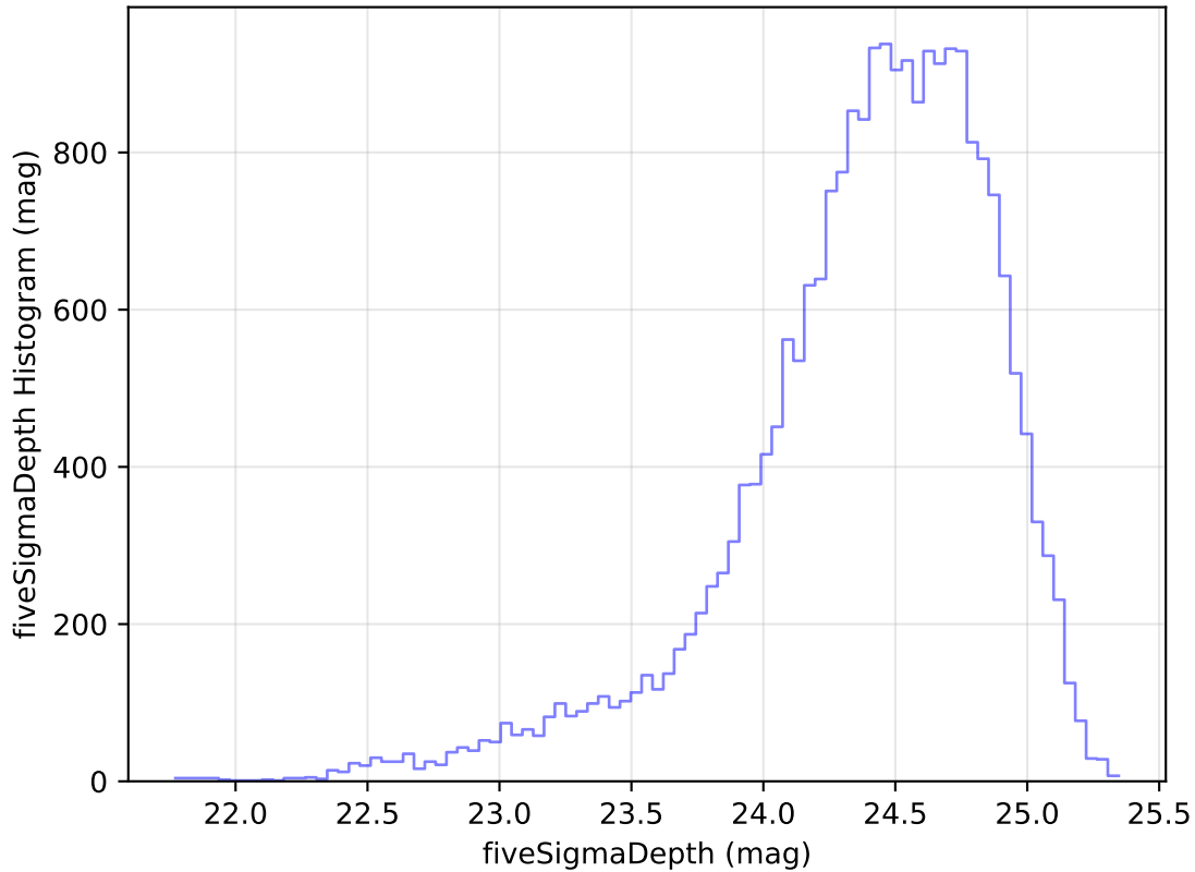
ddf_acor_sf15_lsf40_lsr50_v3.4_10yrs Yr 1 g band: fiveSigmaDepth Histogram
