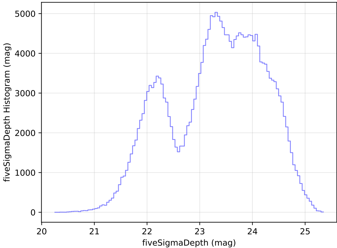
ddf_acor_sf15_lsf40_lsr50_v3.4_10yrs Yr 1 all bands: fiveSigmaDepth Histogram
