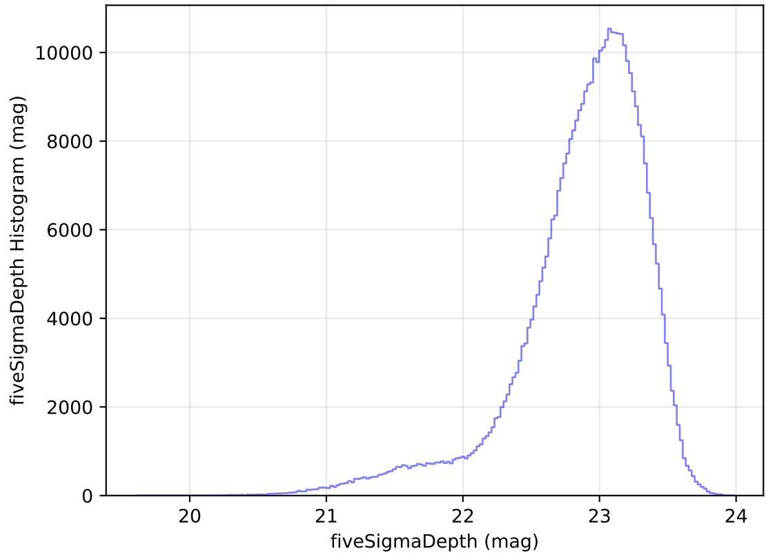
ddf_acor_sf15_lsf40_lsr50_v3.4_10yrs WFD z band: fiveSigmaDepth Histogram
