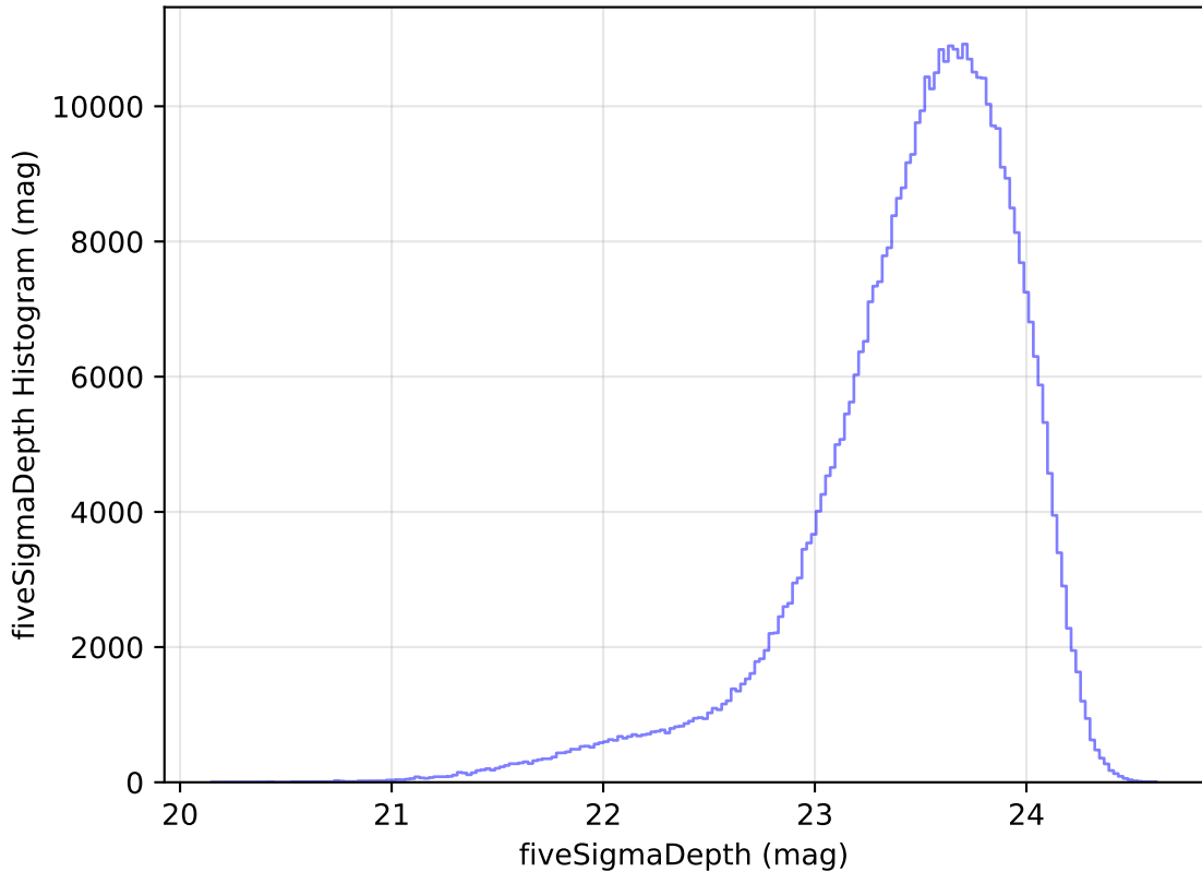
ddf_acor_sf15_lsf40_lsr50_v3.4_10yrs WFD i band: fiveSigmaDepth Histogram
