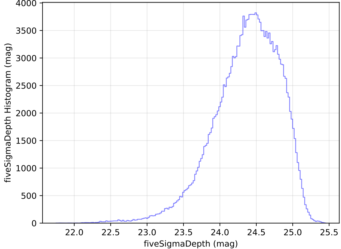
ddf_acor_sf15_lsf40_lsr50_v3.4_10yrs WFD g band: fiveSigmaDepth Histogram
