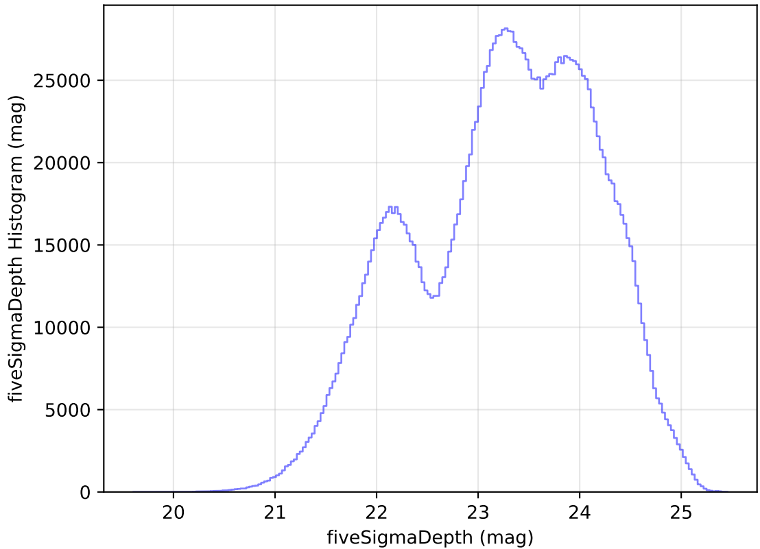
ddf_acor_sf15_lsf40_lsr50_v3.4_10yrs WFD all bands: fiveSigmaDepth Histogram
