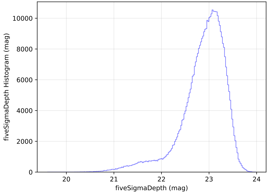
ddf_acor_sf15_lsf40_lsr50_v3.4_10yrs All sky z band: fiveSigmaDepth Histogram
