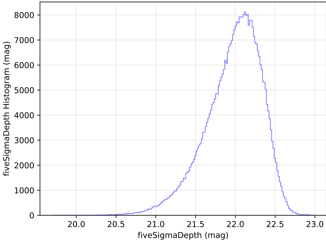
ddf_acor_sf15_lsf40_lsr50_v3.4_10yrs All sky y band: fiveSigmaDepth Histogram
