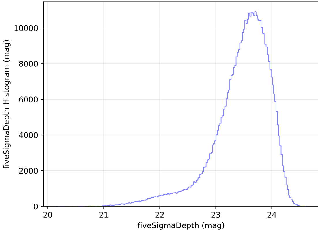
ddf_acor_sf15_lsf40_lsr50_v3.4_10yrs All sky i band: fiveSigmaDepth Histogram
