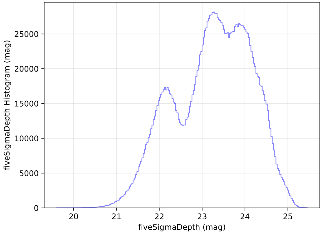
ddf_acor_sf15_lsf40_lsr50_v3.4_10yrs All sky all bands: fiveSigmaDepth Histogram
