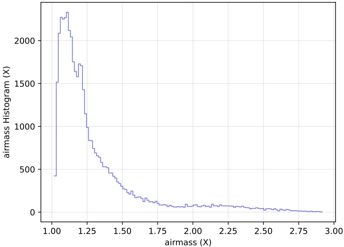
ddf_acor_sf15_lsf40_lsr50_v3.4_10yrs Yr 1 z band: airmass Histogram
