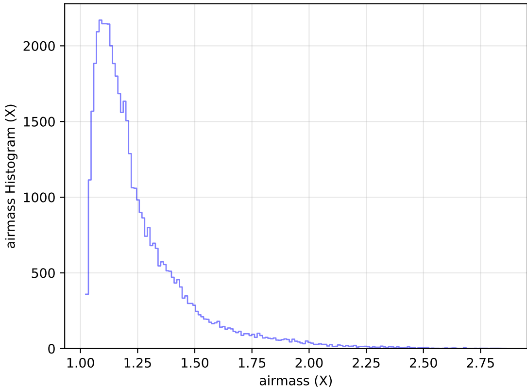
ddf_acor_sf15_lsf40_lsr50_v3.4_10yrs Yr 1 y band: airmass Histogram
