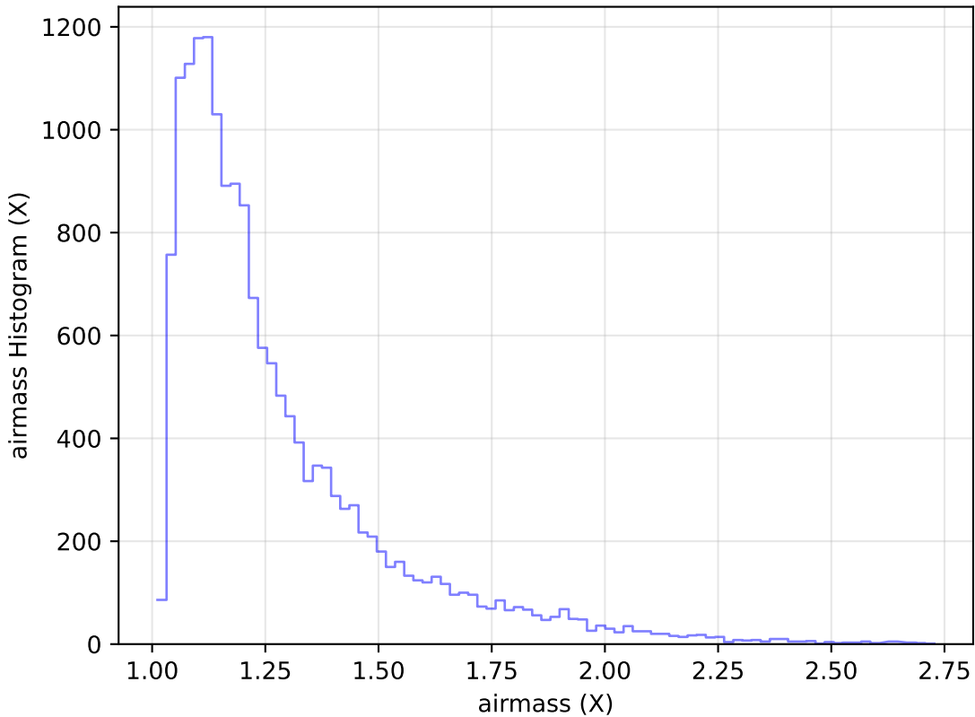
ddf_acor_sf15_lsf40_lsr50_v3.4_10yrs Yr 1 u band: airmass Histogram
