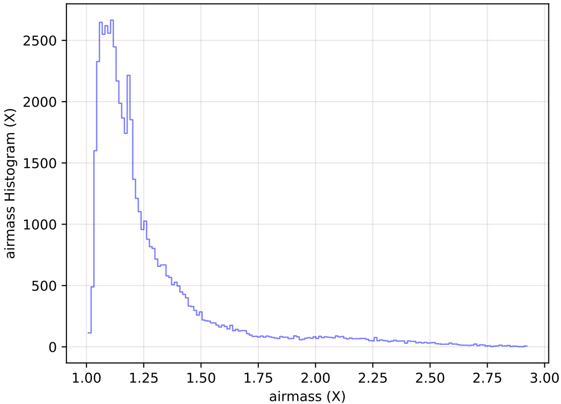
ddf_acor_sf15_lsf40_lsr50_v3.4_10yrs Yr 1 i band: airmass Histogram
