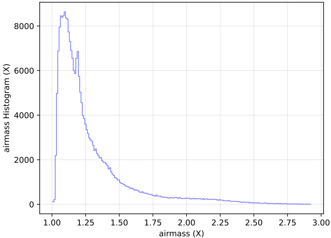
ddf_acor_sf15_lsf40_lsr50_v3.4_10yrs Yr 1 all bands: airmass Histogram
