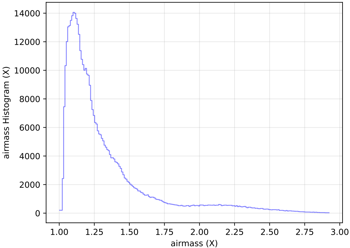
ddf_acor_sf15_lsf40_lsr50_v3.4_10yrs WFD z band: airmass Histogram
