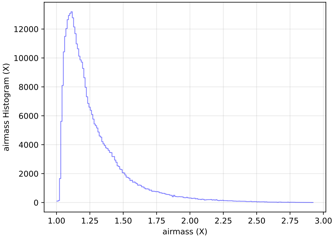
ddf_acor_sf15_lsf40_lsr50_v3.4_10yrs WFD y band: airmass Histogram
