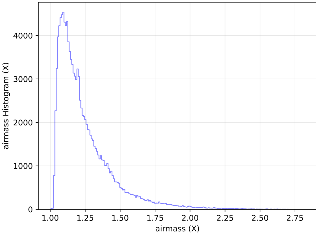
ddf_acor_sf15_lsf40_lsr50_v3.4_10yrs WFD u band: airmass Histogram
