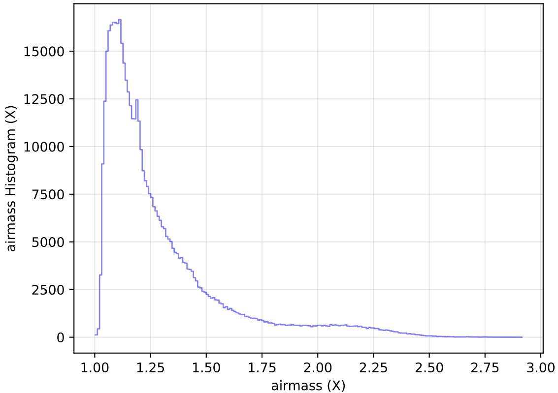
ddf_acor_sf15_Isf40_Isr50_v3.4_10yrs WFD r band: airmass Histogram
