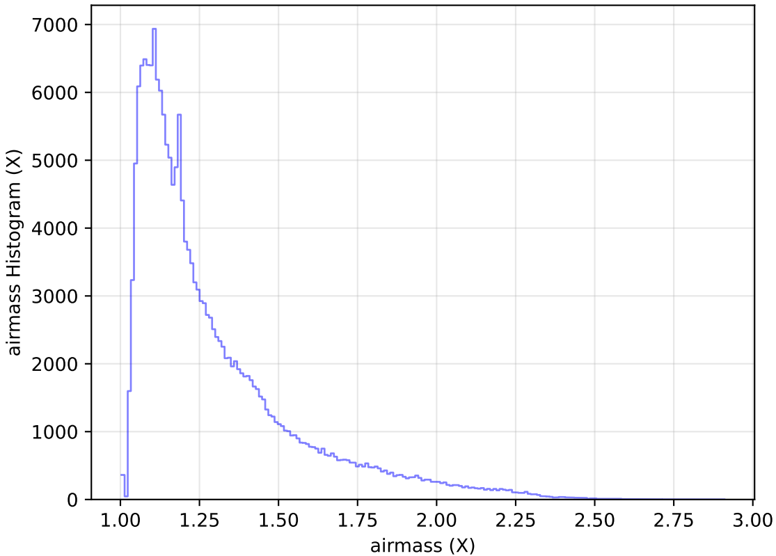
ddf_acor_sf15_lsf40_lsr50_v3.4_10yrs WFD g band: airmass Histogram
