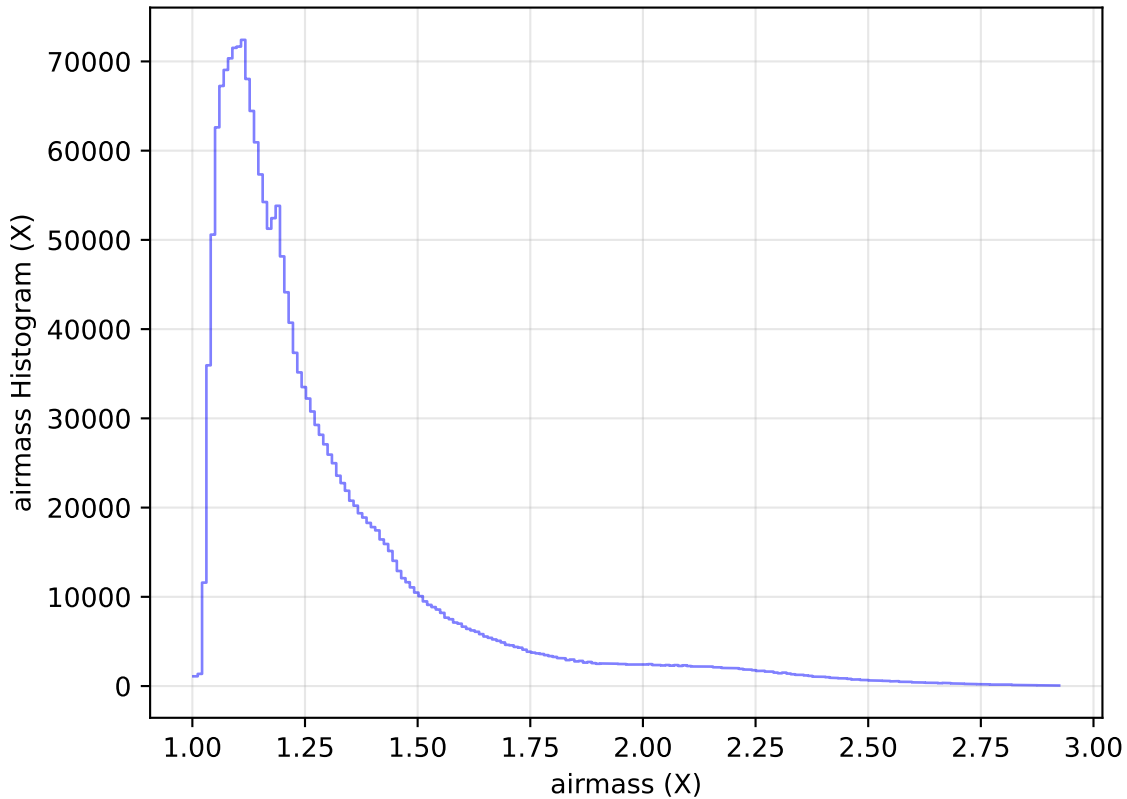
ddf_acor_sf15_lsf40_lsr50_v3.4_10yrs WFD all bands: airmass Histogram
