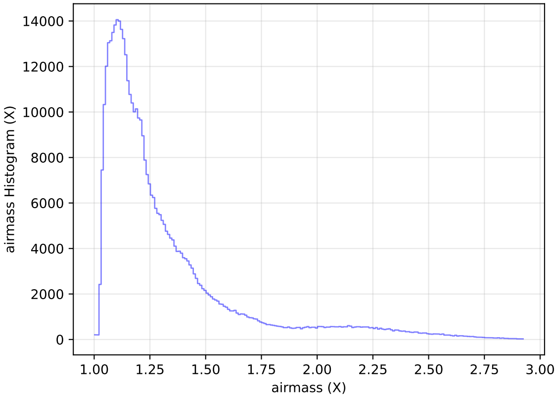
ddf_acor_sf15_lsf40_lsr50_v3.4_10yrs All sky z band: airmass Histogram
