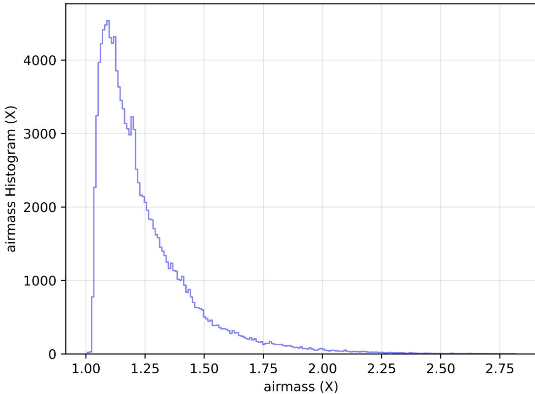
ddf_acor_sf15_lsf40_lsr50_v3.4_10yrs All sky u band: airmass Histogram
