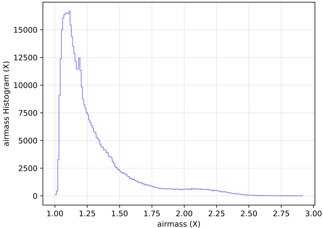
ddf_acor_sf15_lsf40_lsr50_v3.4_10yrs All sky r band: airmass Histogram
