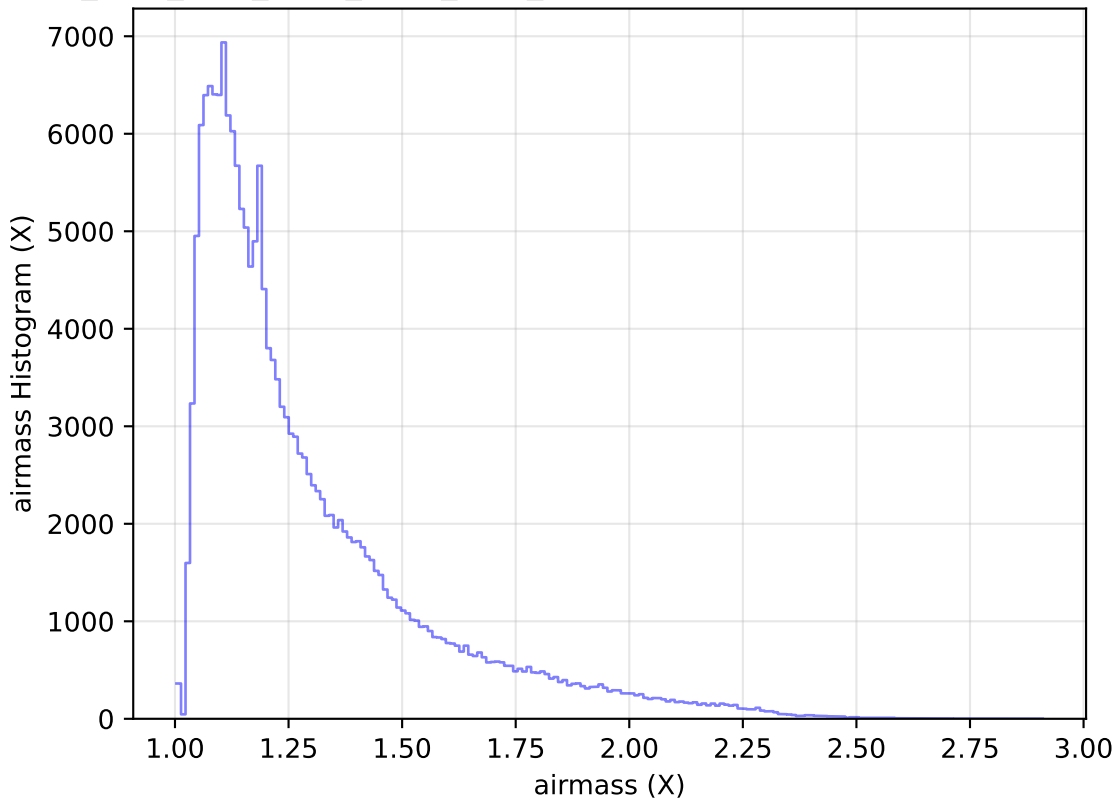
ddf_acor_sf15_lsf40_lsr50_v3.4_10yrs All sky g band: airmass Histogram
