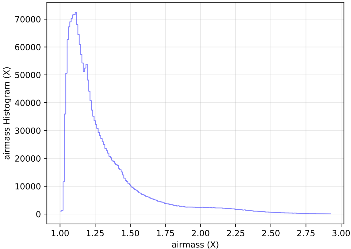
ddf_acor_sf15_lsf40_lsr50_v3.4_10yrs All sky all bands: airmass Histogram
