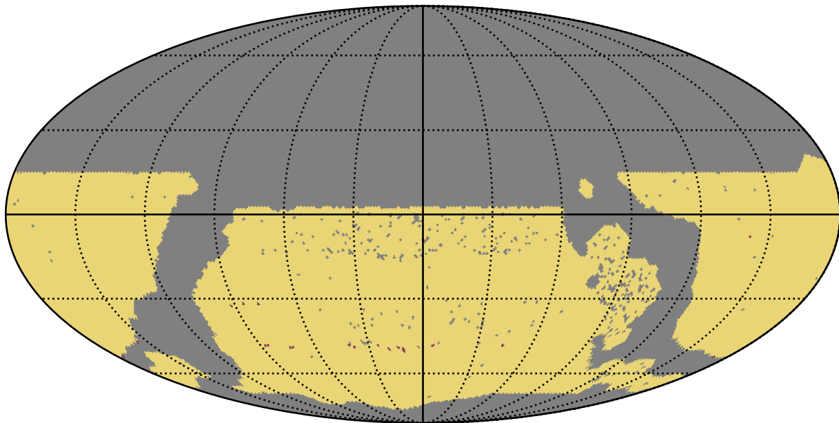
ddf_acor_sf15_lsf40_lsr50_v3.4_10yrs WFD: RapidRevisits
