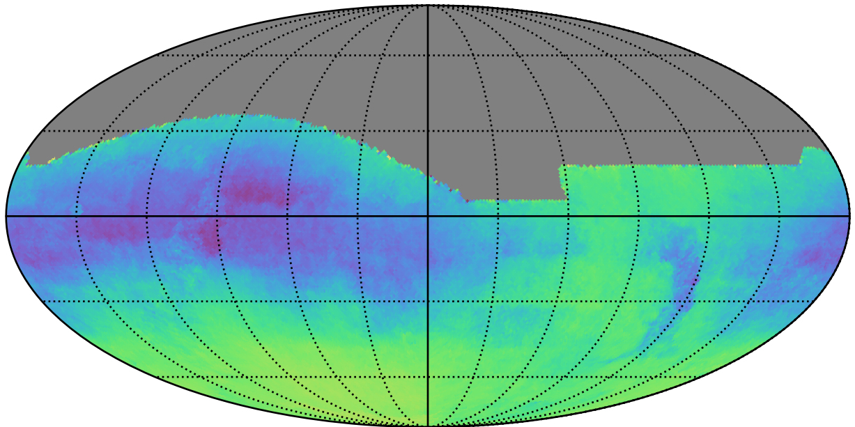
ddf_acor_sf15_lsf40_lsr50_v3.4_10yrs All sky: Parallax-DCR degeneracy @ 24.0
